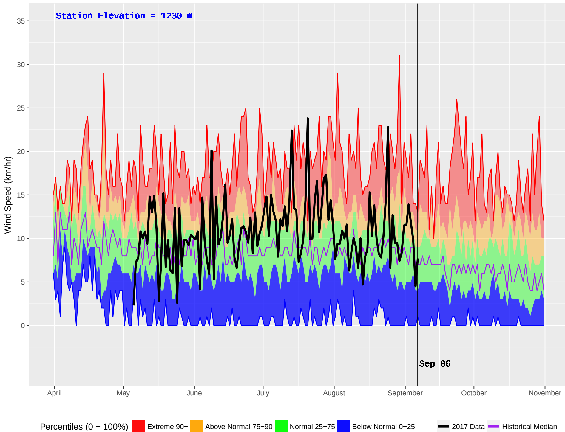
SLOCAN (406) : Historical (1992–2016) and Current (2017) Noon Wind Speed
