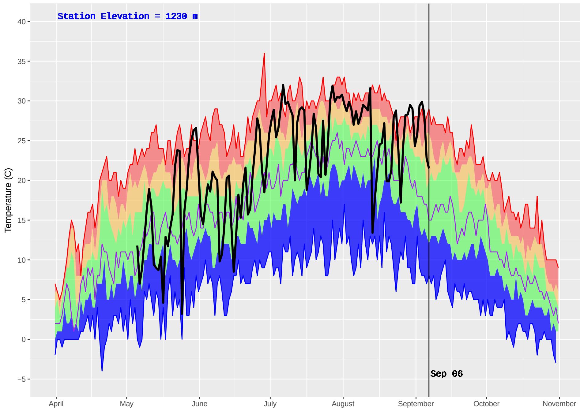
SLOCAN (406) : Historical (1992–2016) and Current (2017) Noon Temperature
