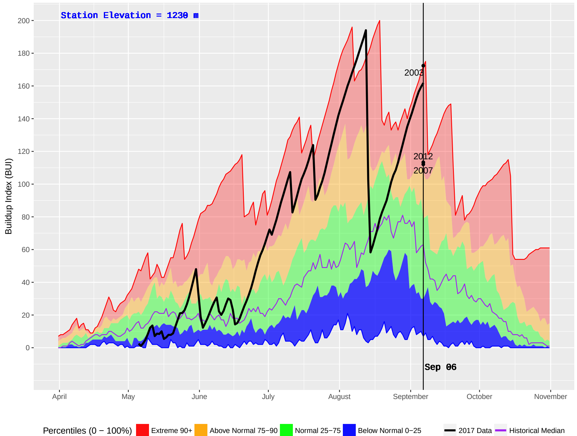
SLOCAN (406) : Historical (1992–2016) and Current (2017) Noon Buildup Index (BUI)
