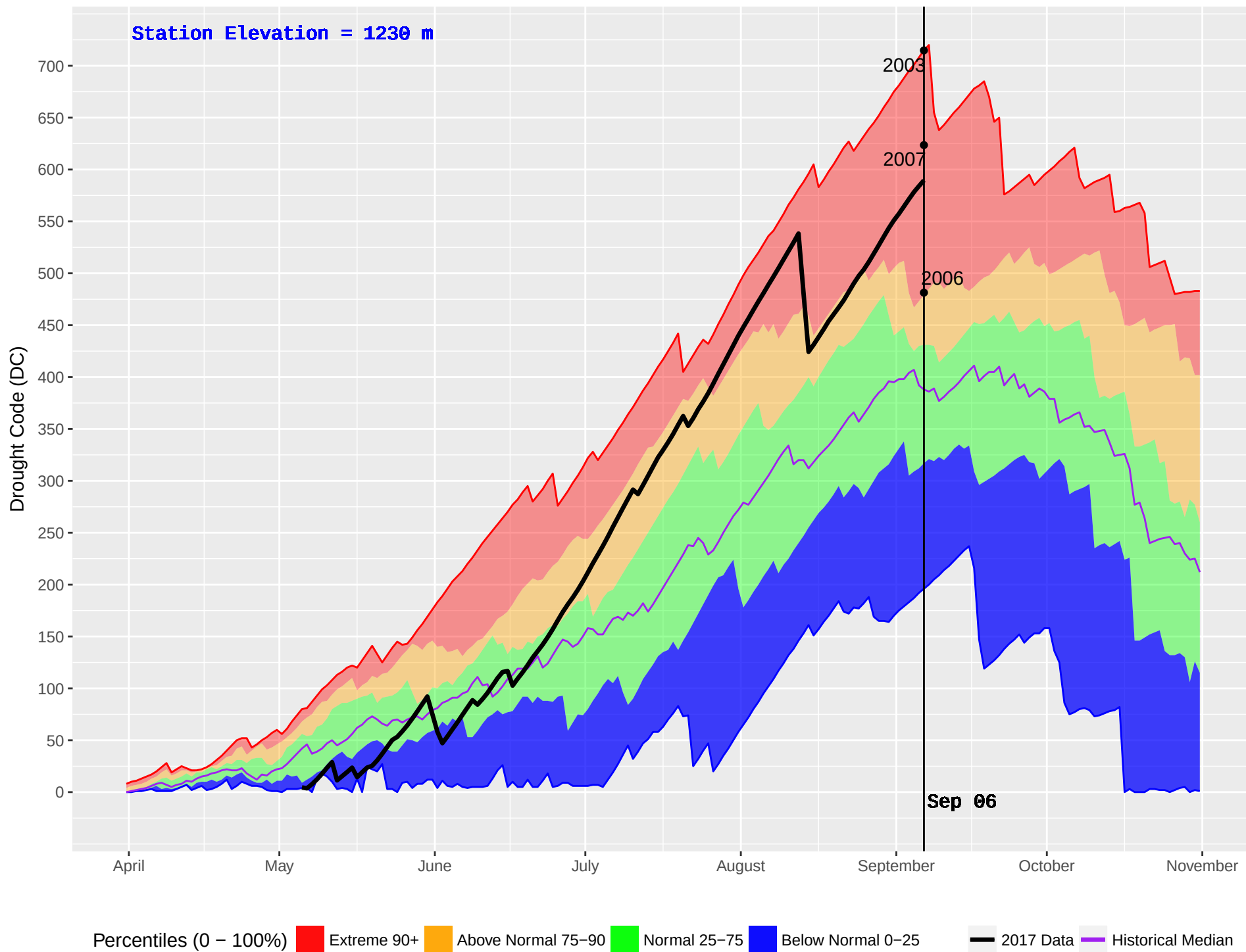
SLOCAN (406) : Historical (1992–2016) and Current (2017) Noon Drought Code (DC)
