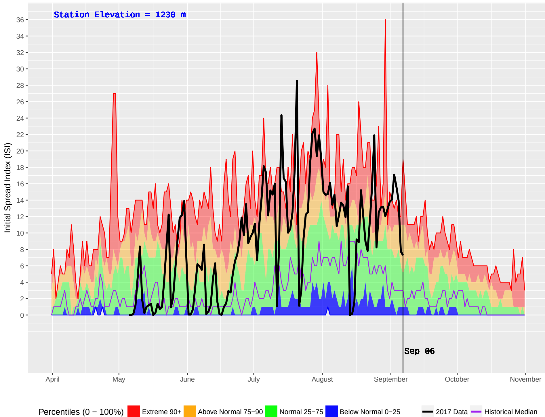
SLOCAN (406) : Historical (1992–2016) and Current (2017) Noon Initial Spread Index (ISI)
