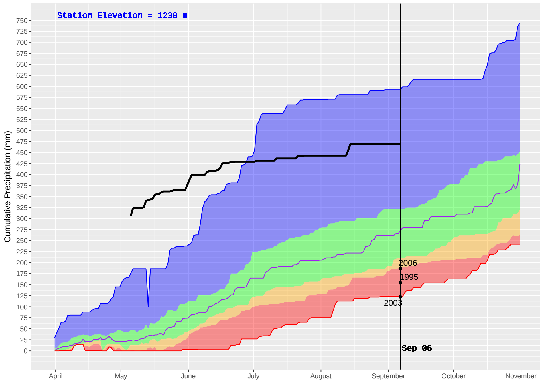
SLOCAN (406) : Historical (1992–2016) and Current (2017) Noon Cumulative Precipitation
