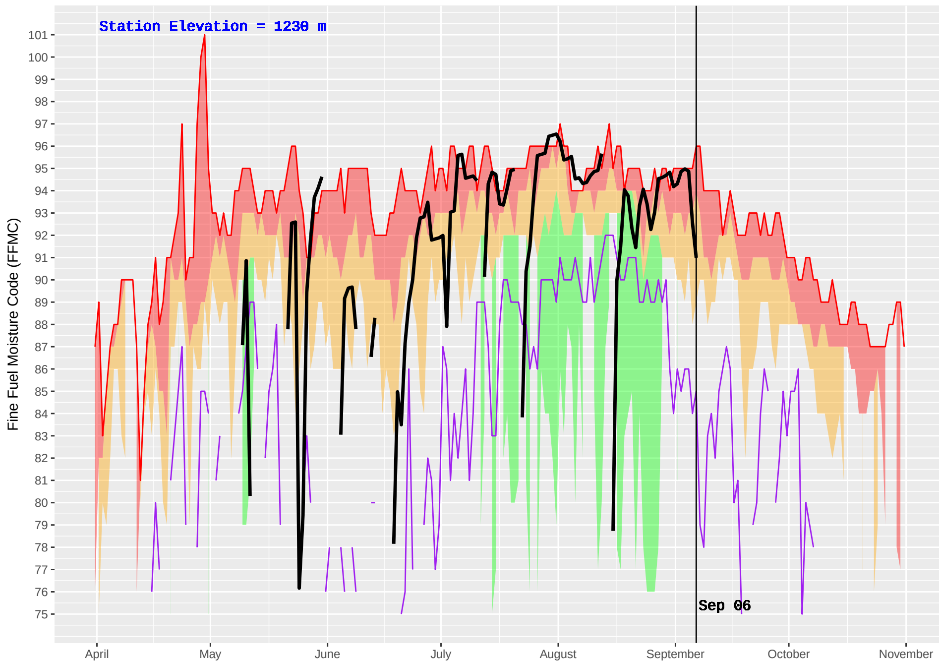
SLOCAN (406) : Historical (1992–2016) and Current (2017) Noon Fine Fuel Moisture Code (FFMC)
